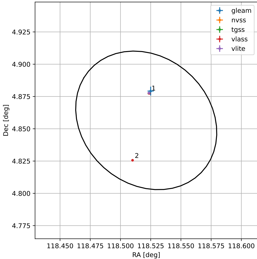
4FGL J0754.0+0451
