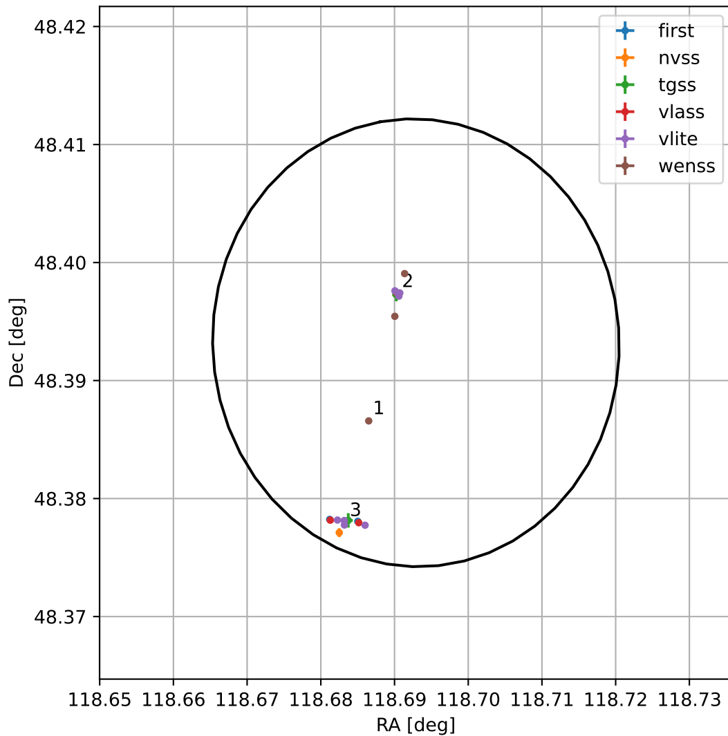
4FGL J0754.7+4823
