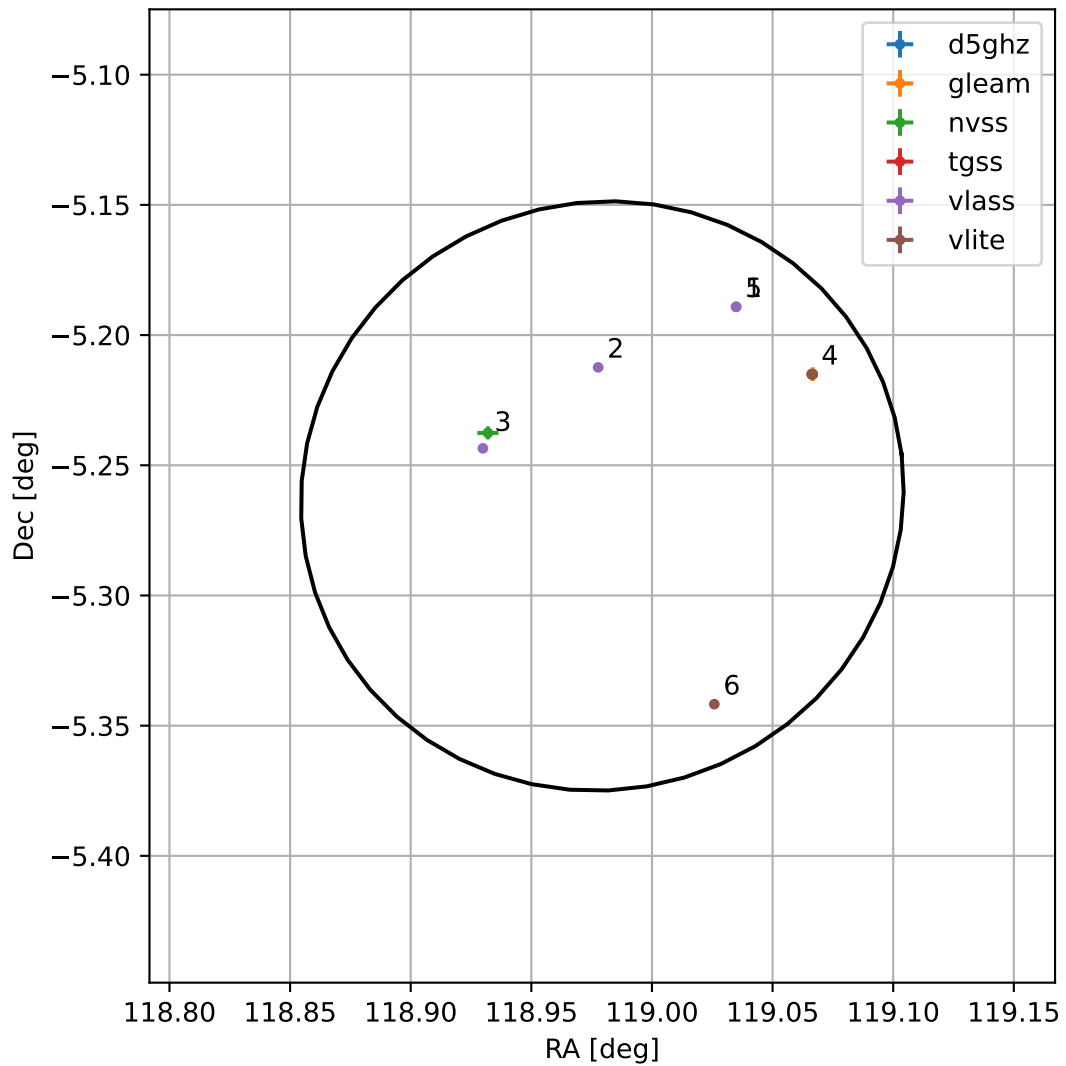
4FGL J0755.9-0515
