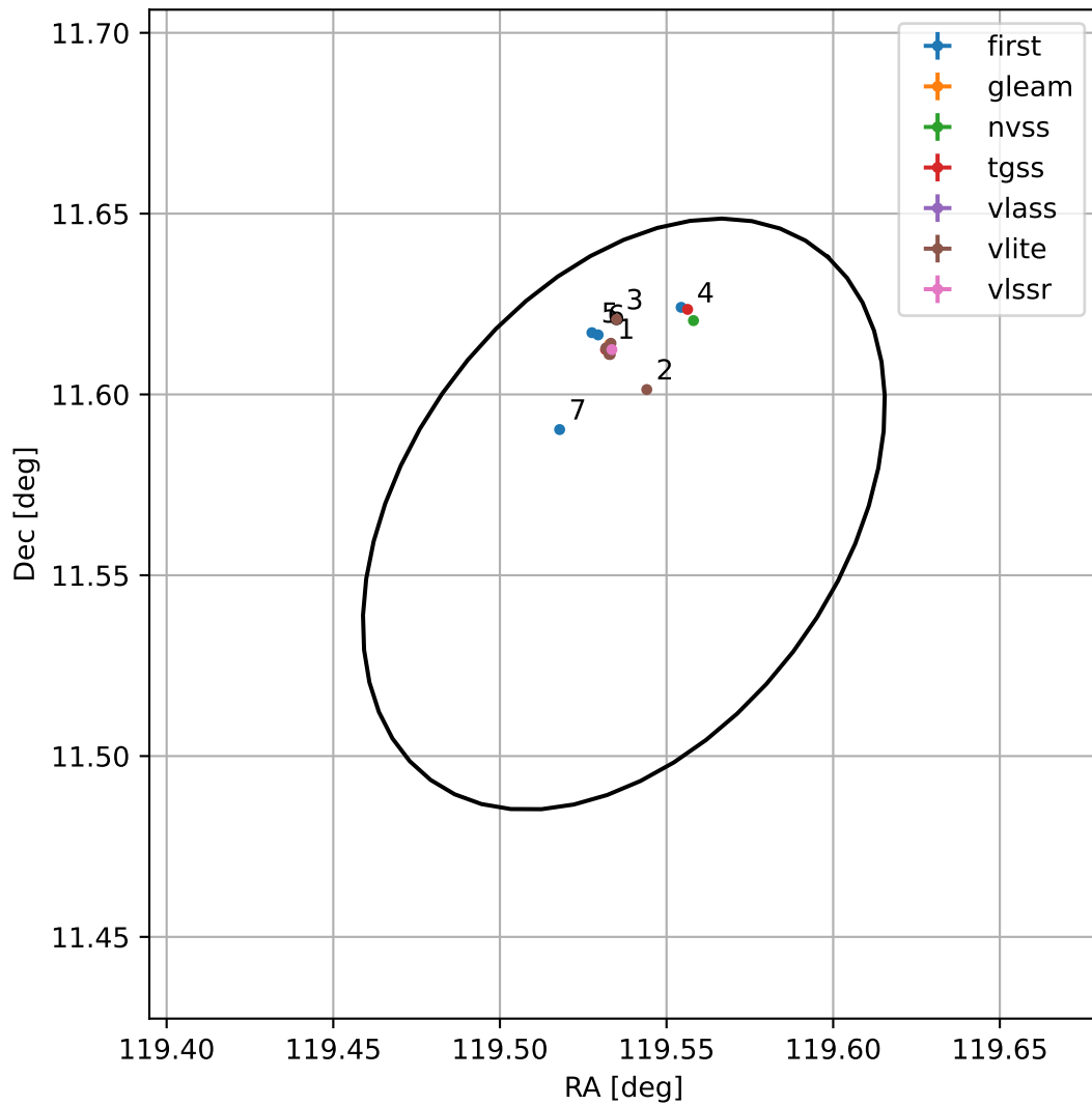
4FGL J0758.1+1134
