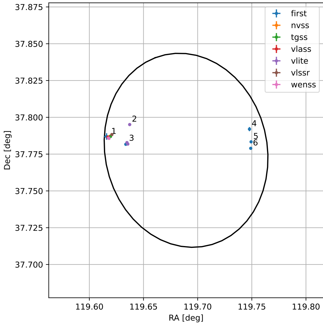
4FGL J0758.7+3746
