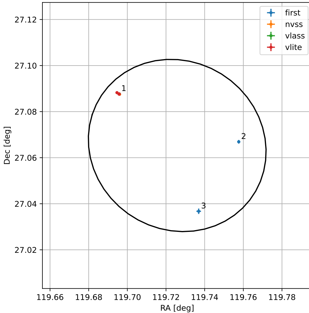
4FGL J0758.9+2703
