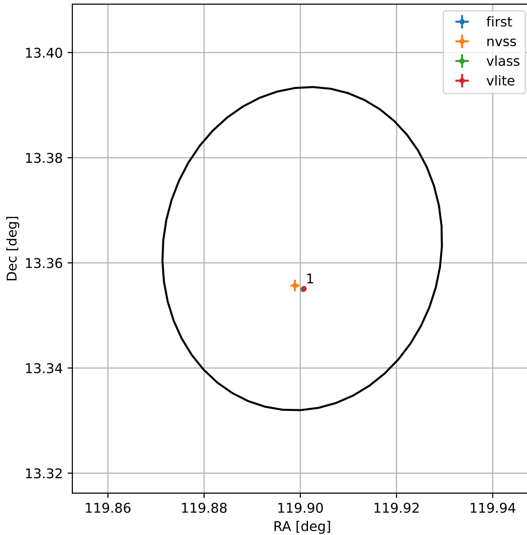
4FGL J0759.6+1321
