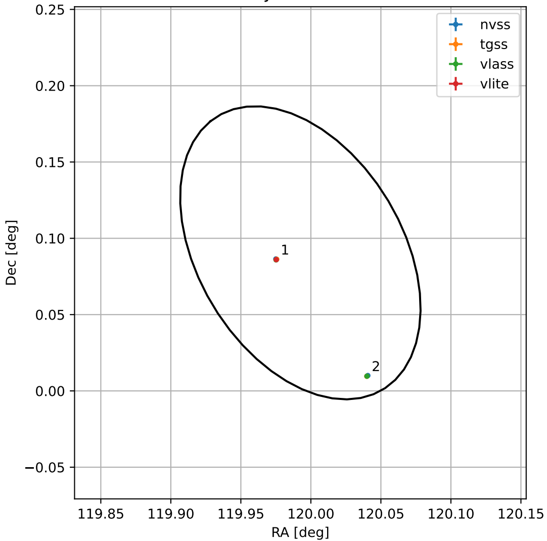
4FGL J0759.9+0005
