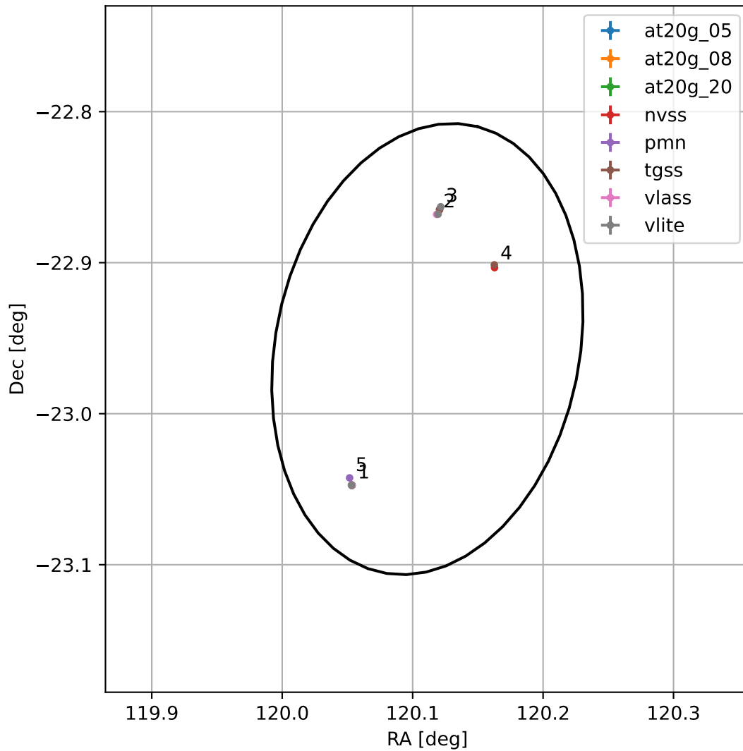
4FGL J0800.4-2257
