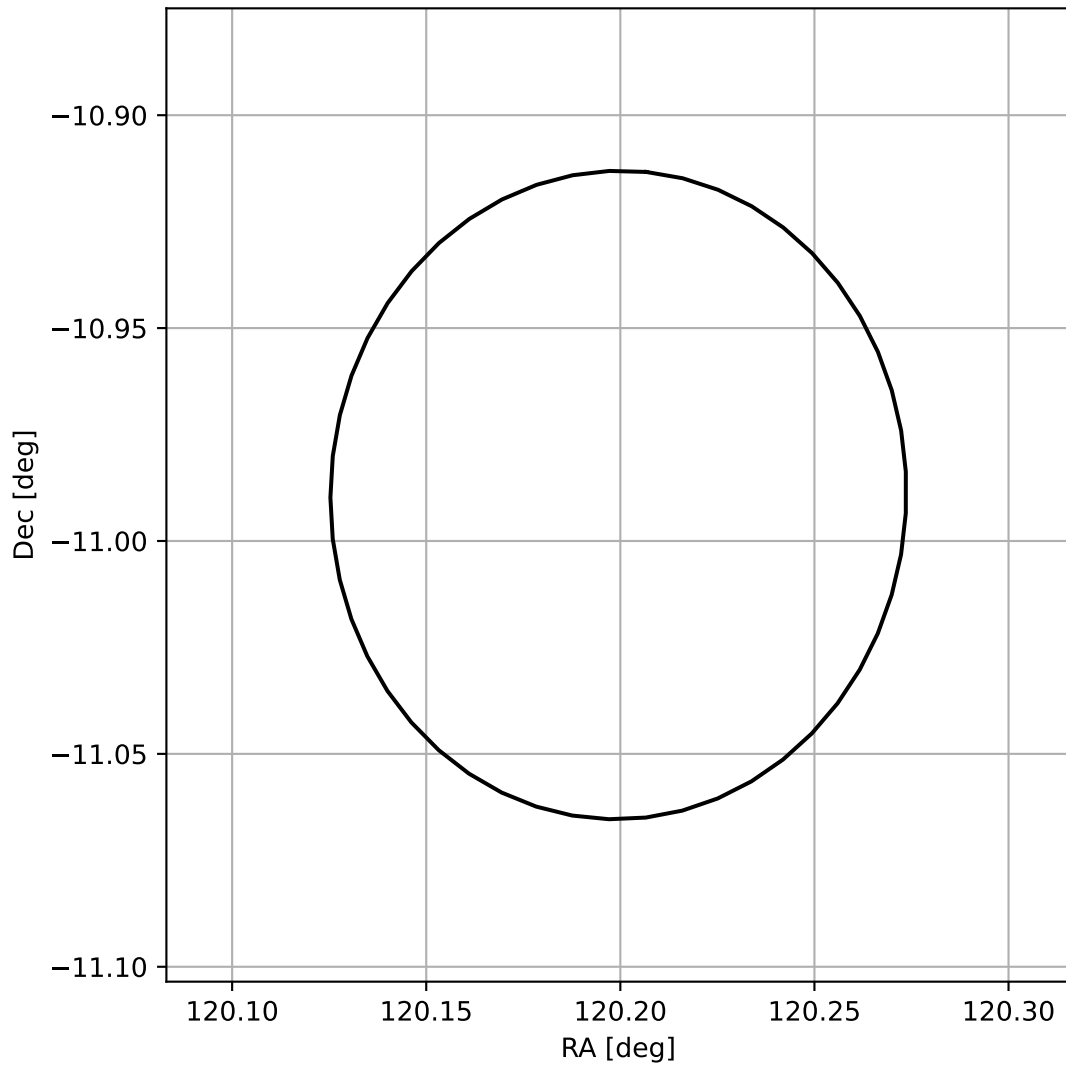
4FGL J0800.7-1059
