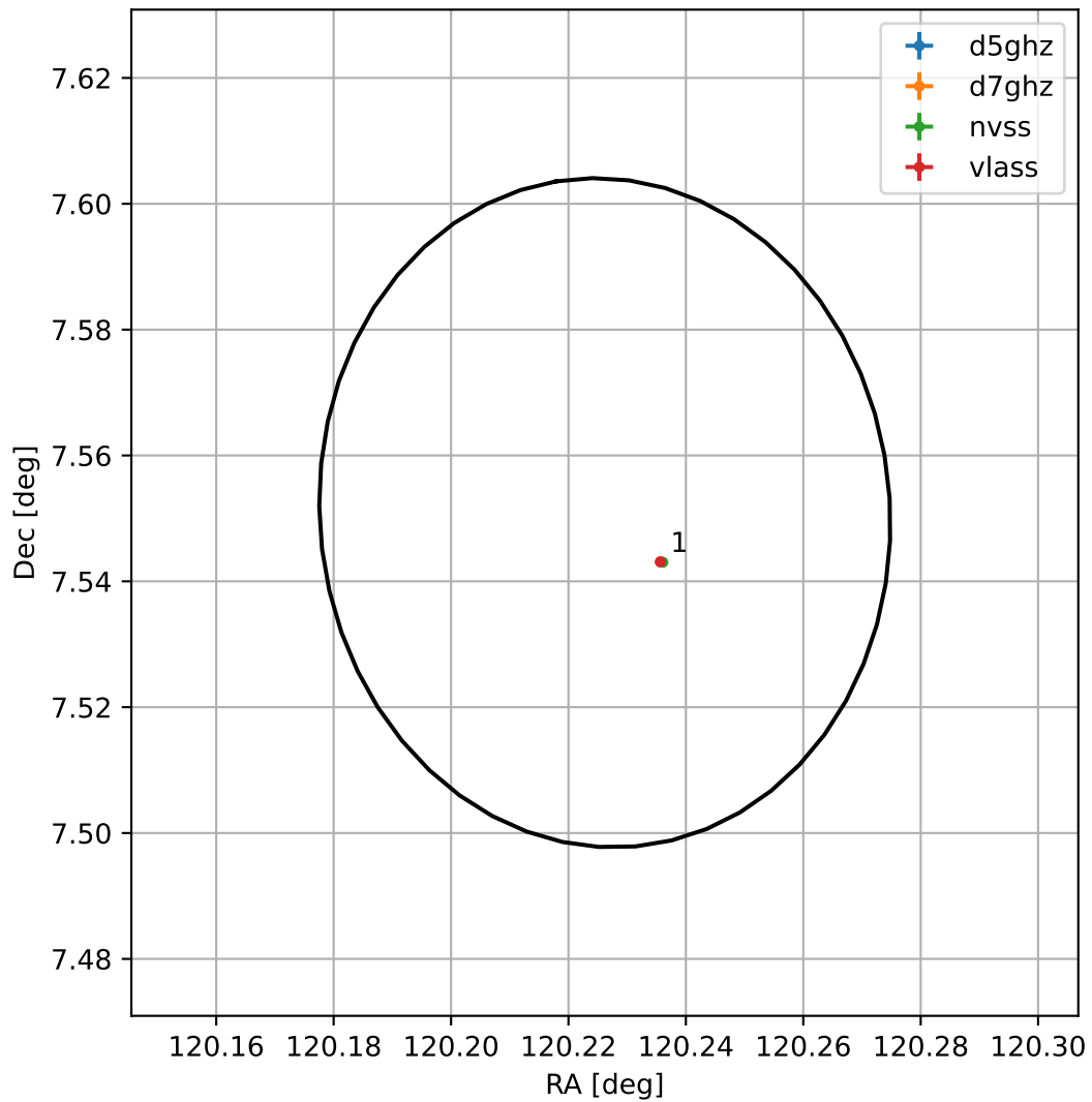
4FGL J0800.9+0733
