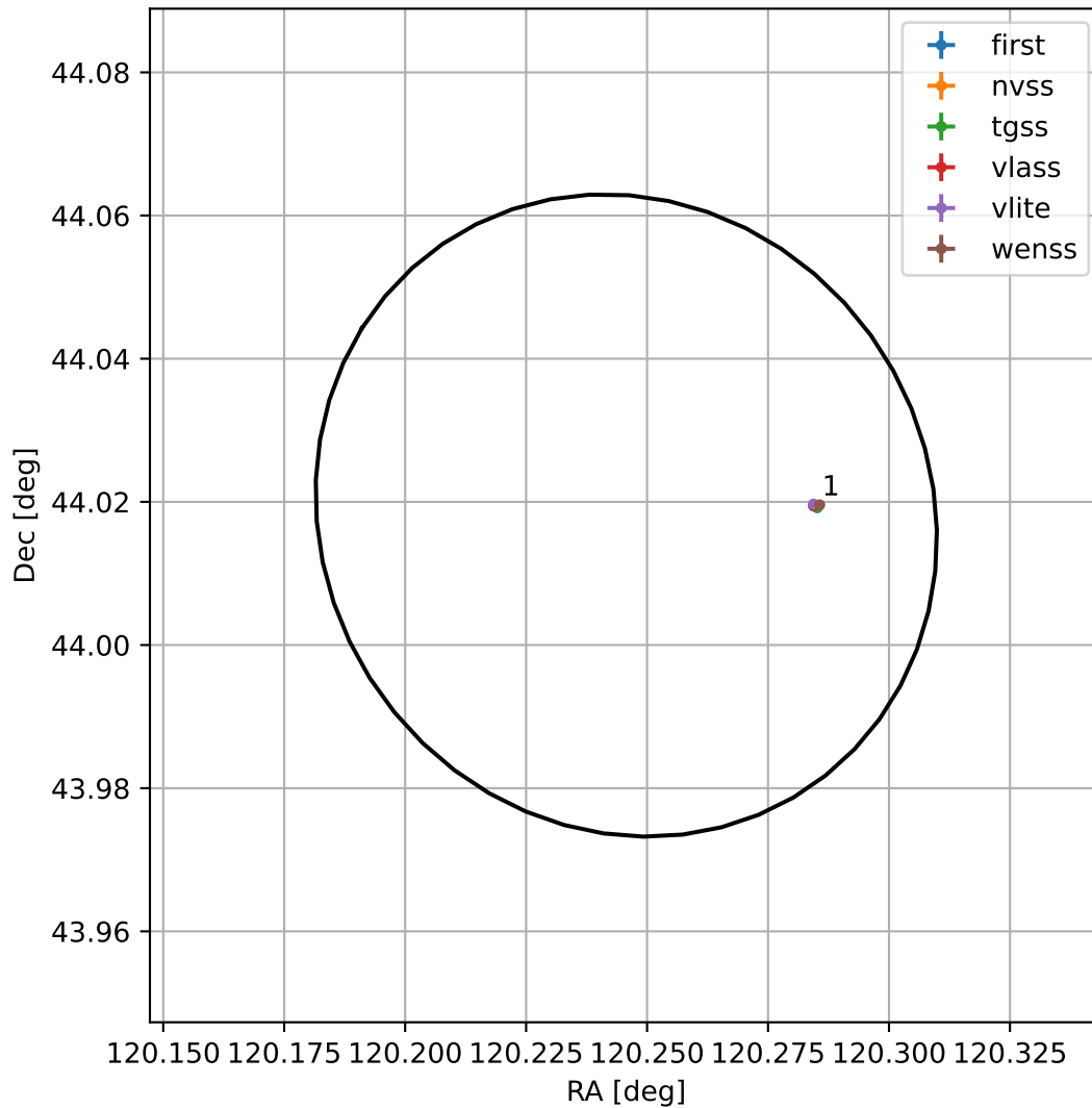
4FGL J0800.9+4401
