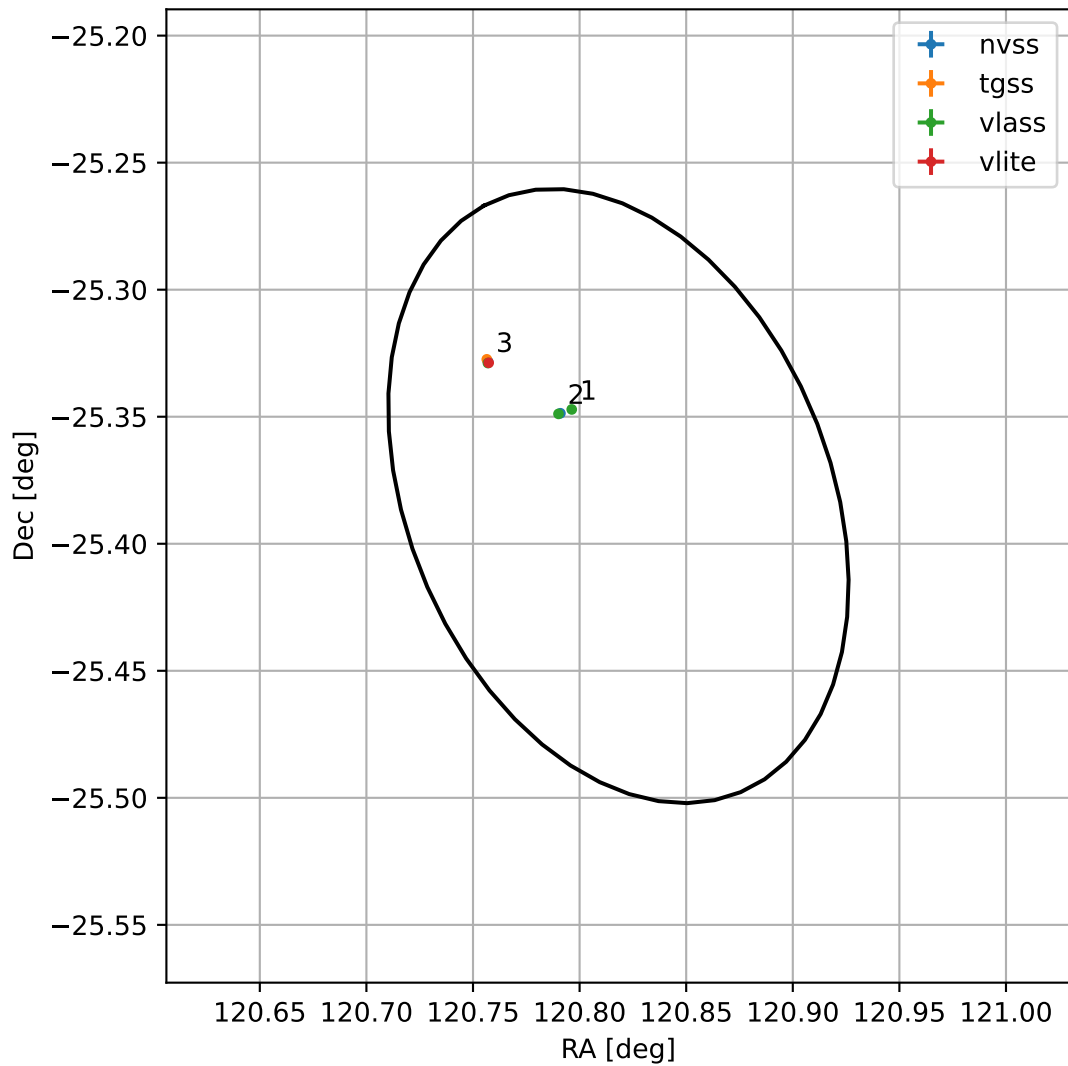
4FGL J0803.2-2522
