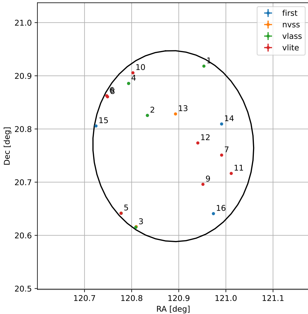
4FGL J0803.5+2046
