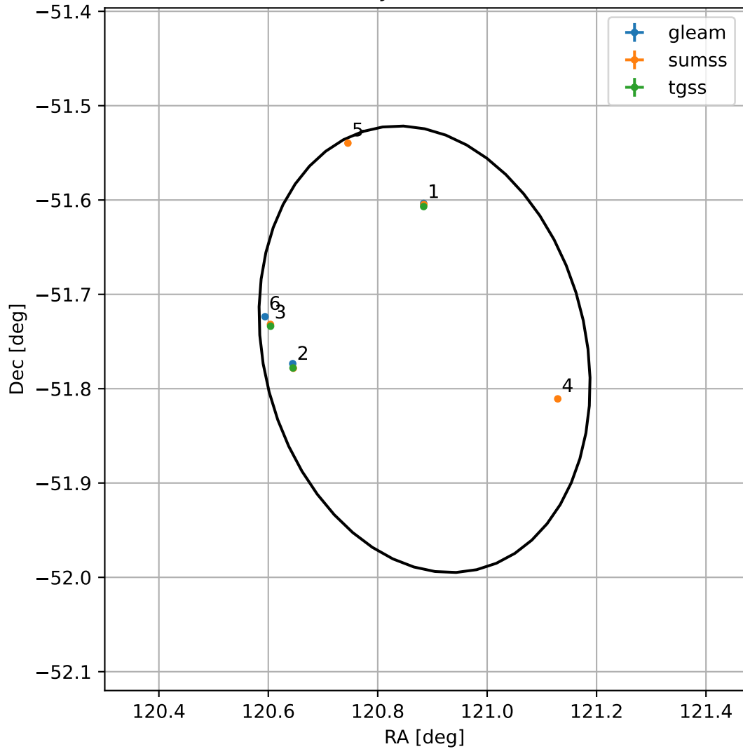
4FGL J0803.5-5145
