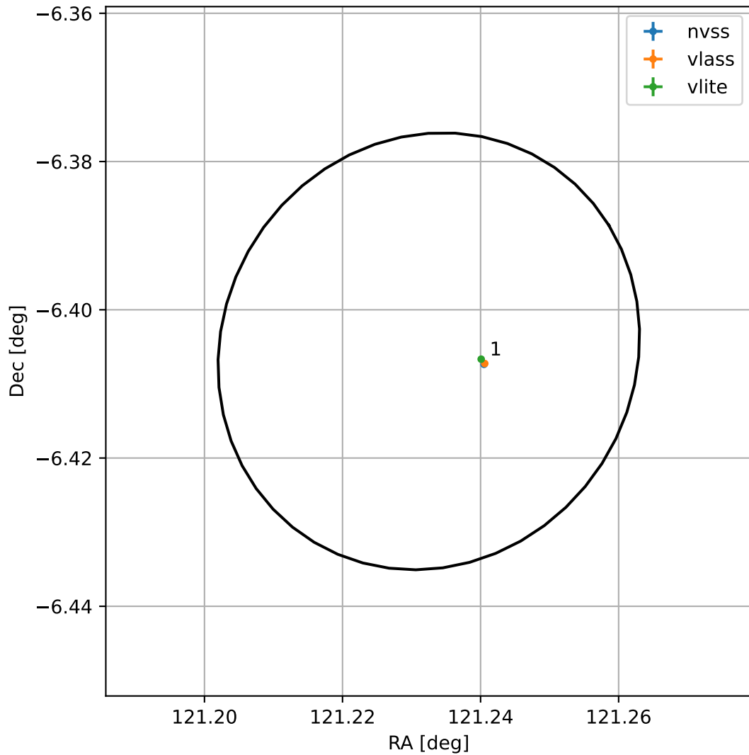
4FGL J0804.9-0624
