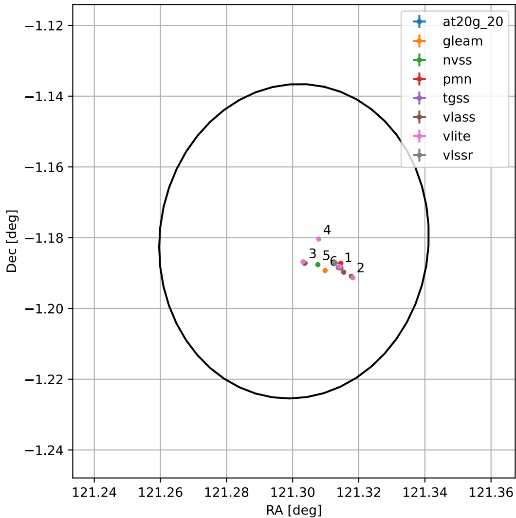
4FGL J0805.2-0110
