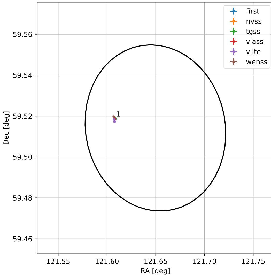
4FGL J0806.5+5930
