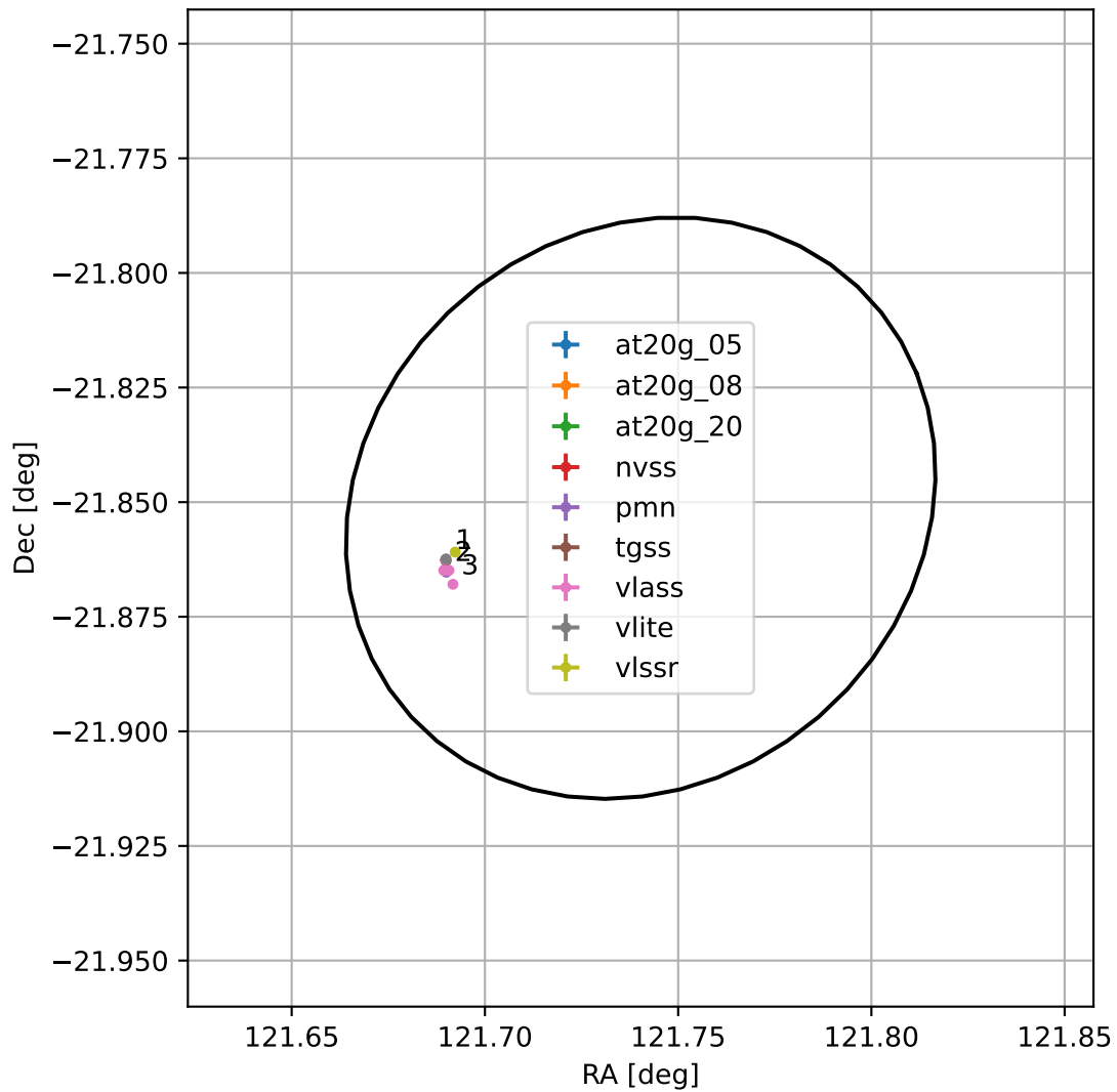
4FGL J0806.9-2151
