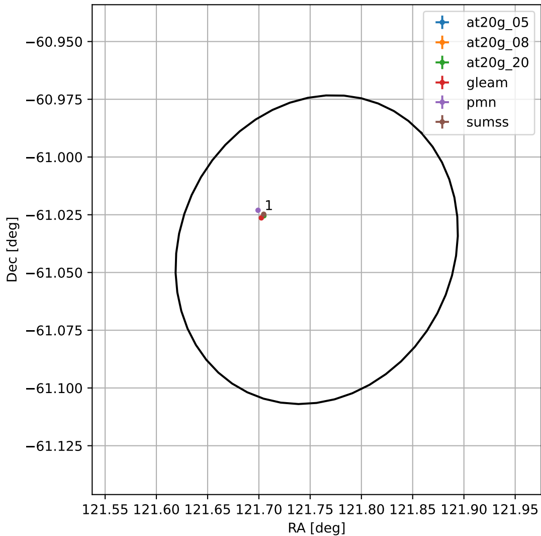
4FGL J0807.0-6102
