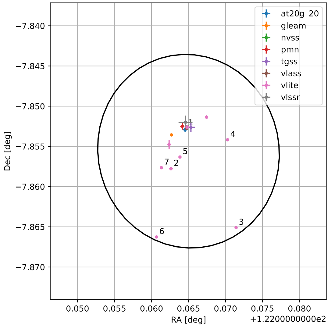
4FGL J0808.2-0751
