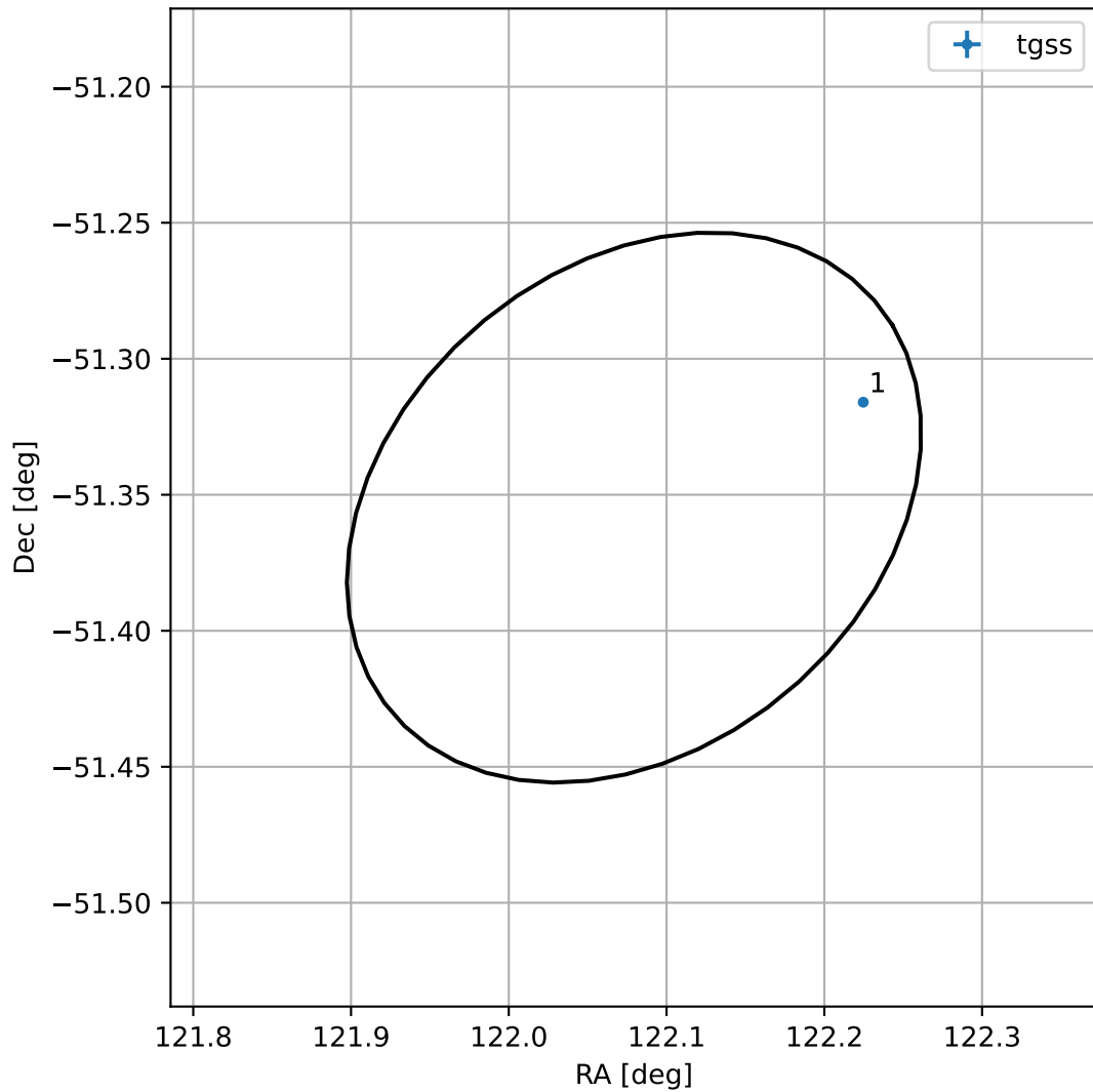
4FGL J0808.3-5121
