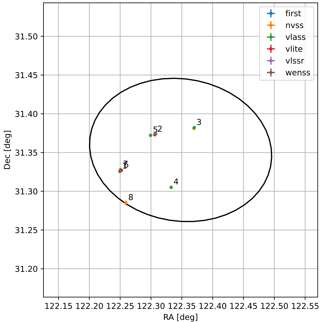
4FGL J0809.3+3121
