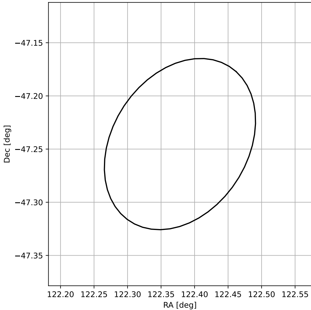
4FGL J0809.5-4714
