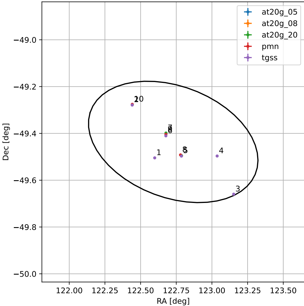
4FGL J0810.9-4926
