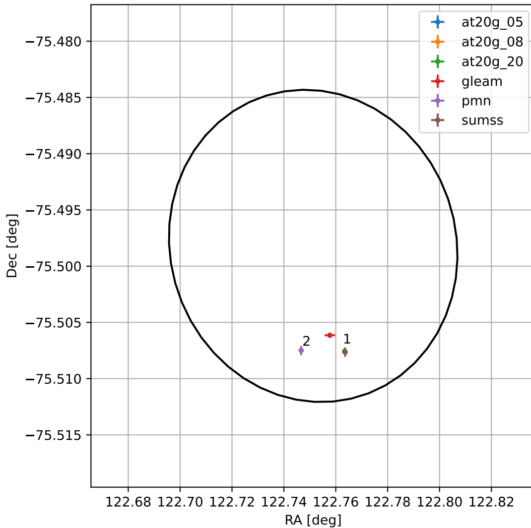
4FGL J0811.0-7529
