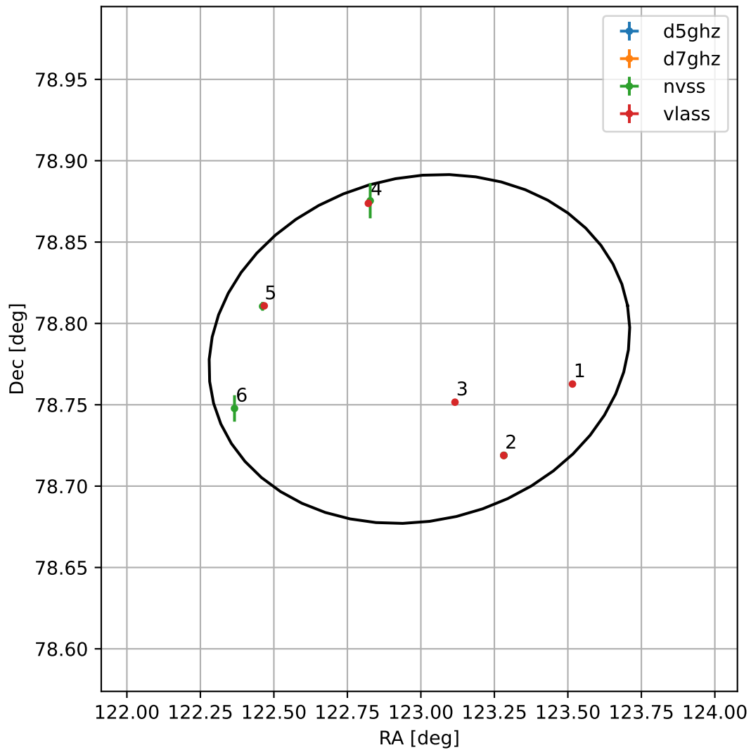
4FGL J0811.9+7847
