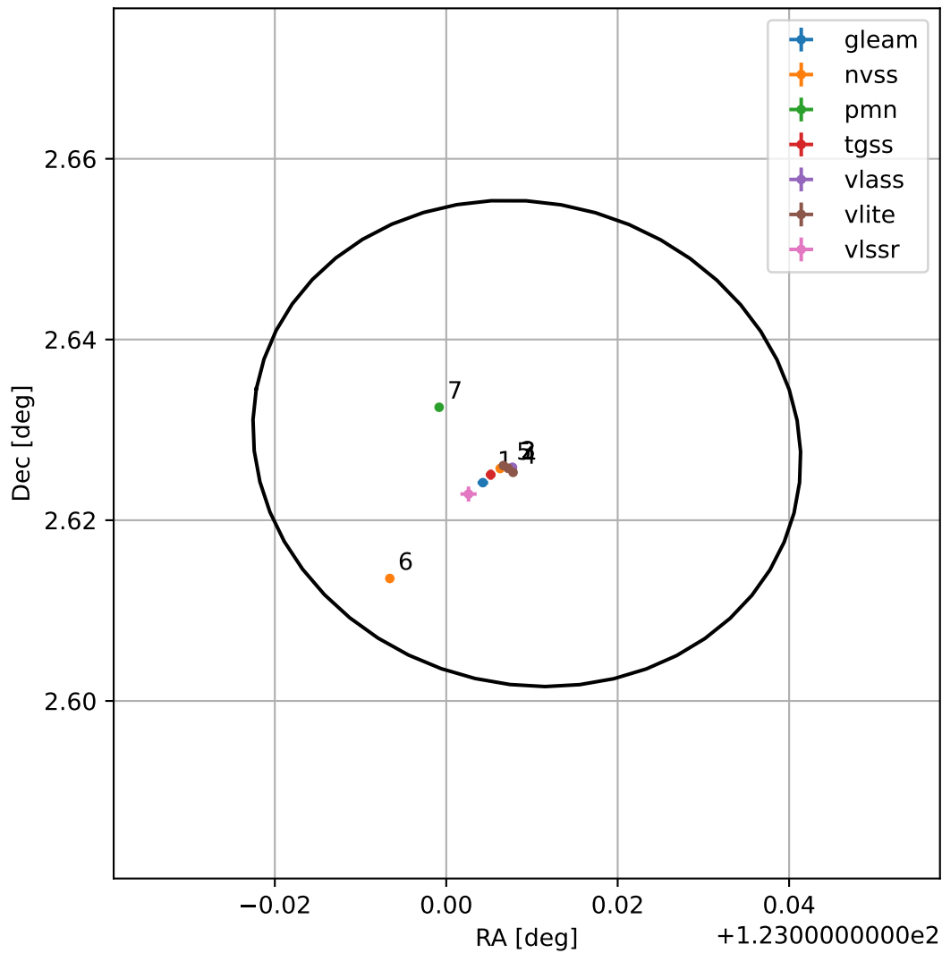
4FGL J0812.0+0237
