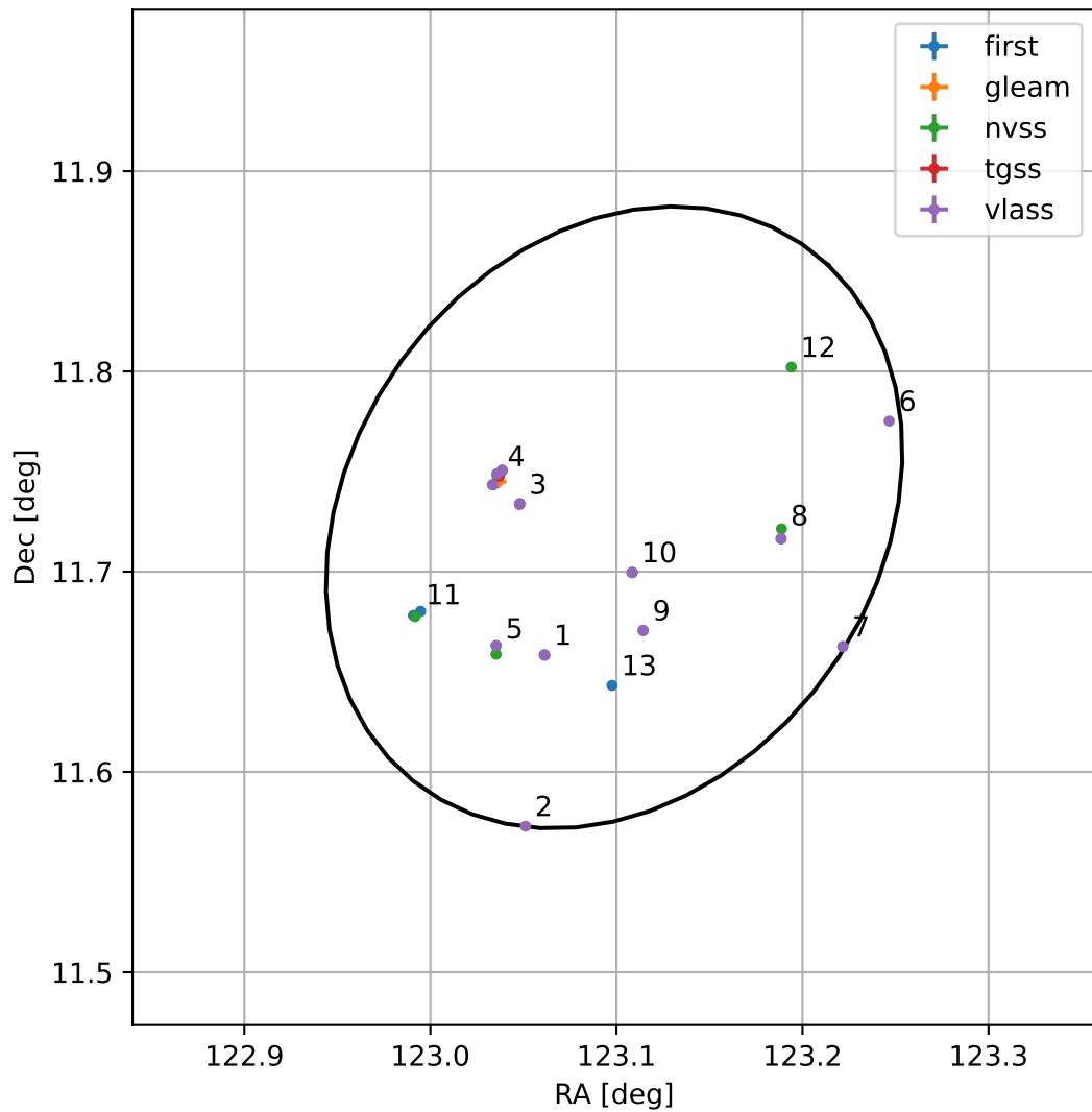
4FGL J0812.3+1143
