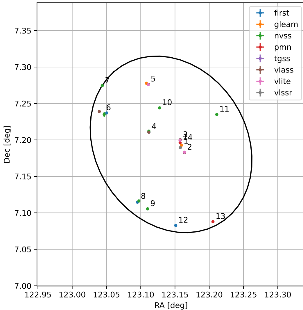
4FGL J0812.5+0711
