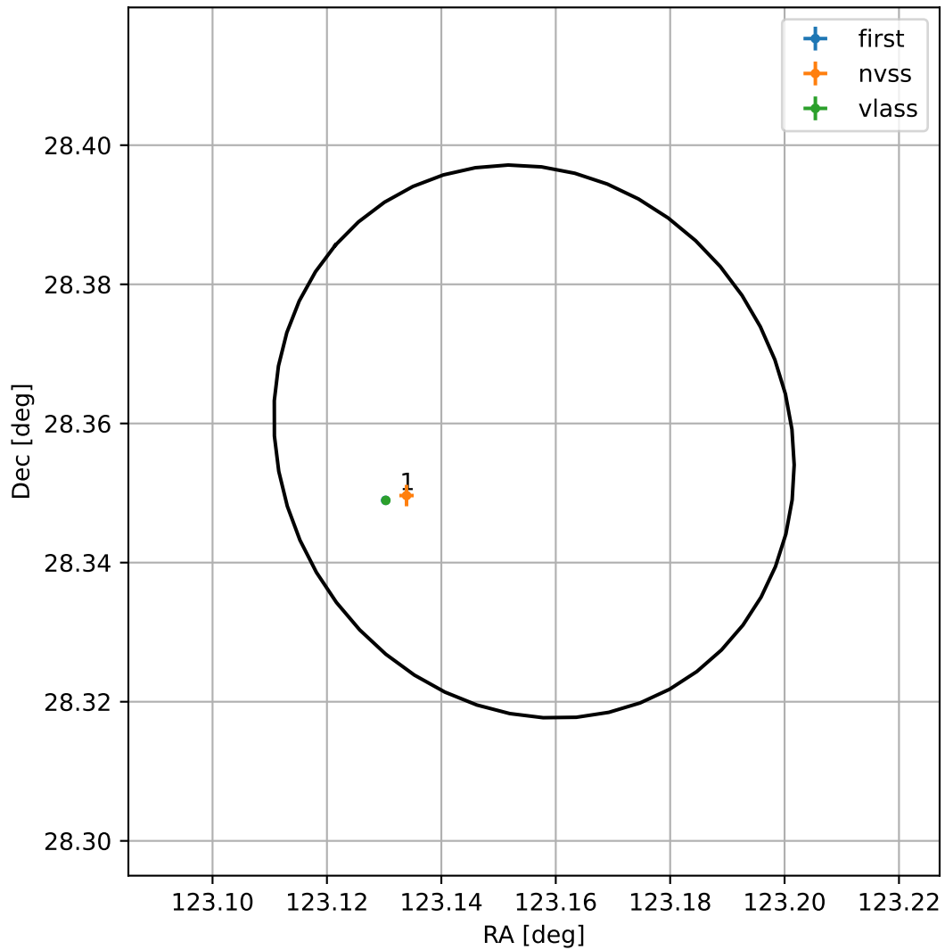
4FGL J0812.6+2821
