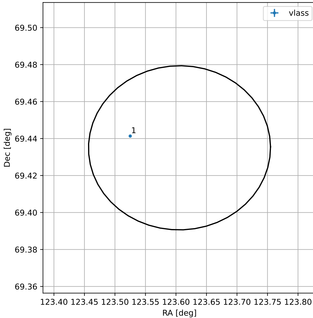
4FGL J0814.4+6926
