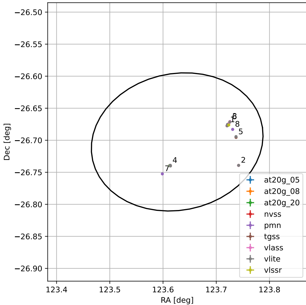
4FGL J0814.5-2642
