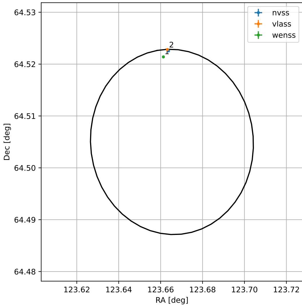
4FGL J0814.6+6430
