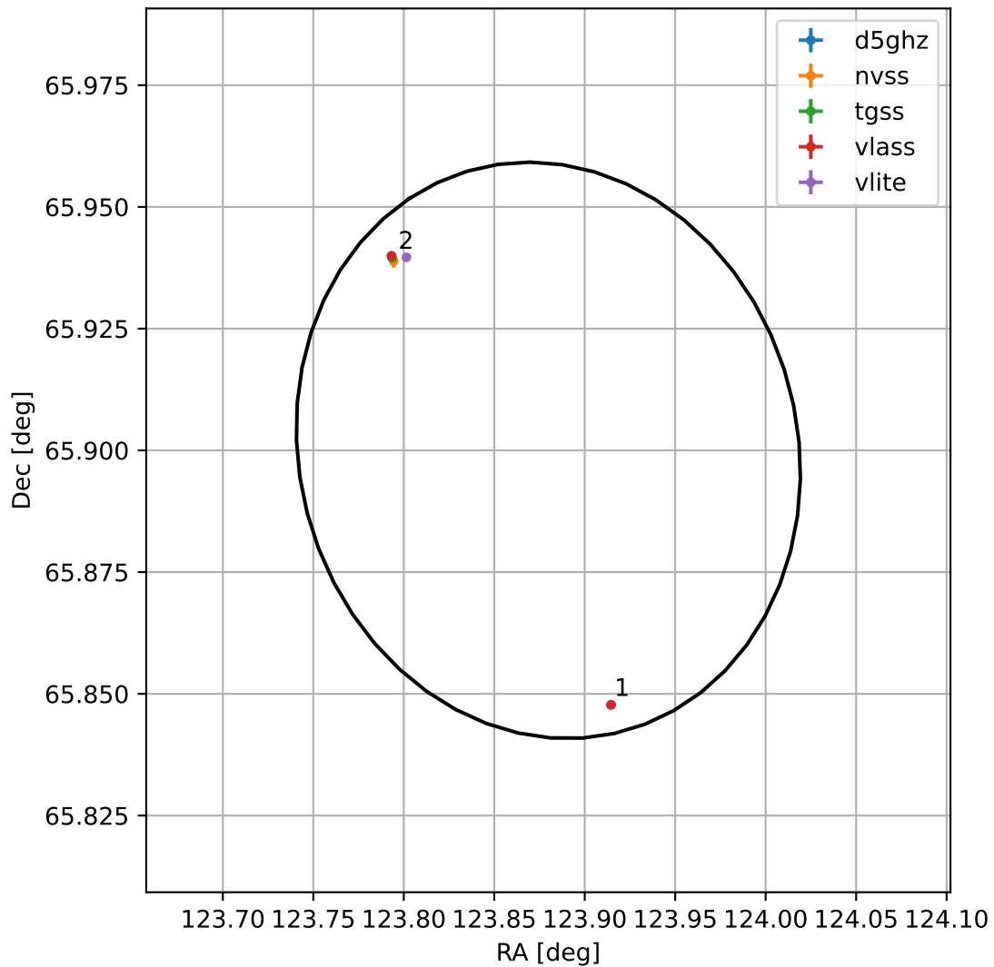
4FGL J0815.5+6554
