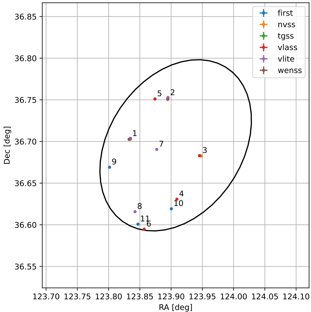
4FGL J0815.6+3641
