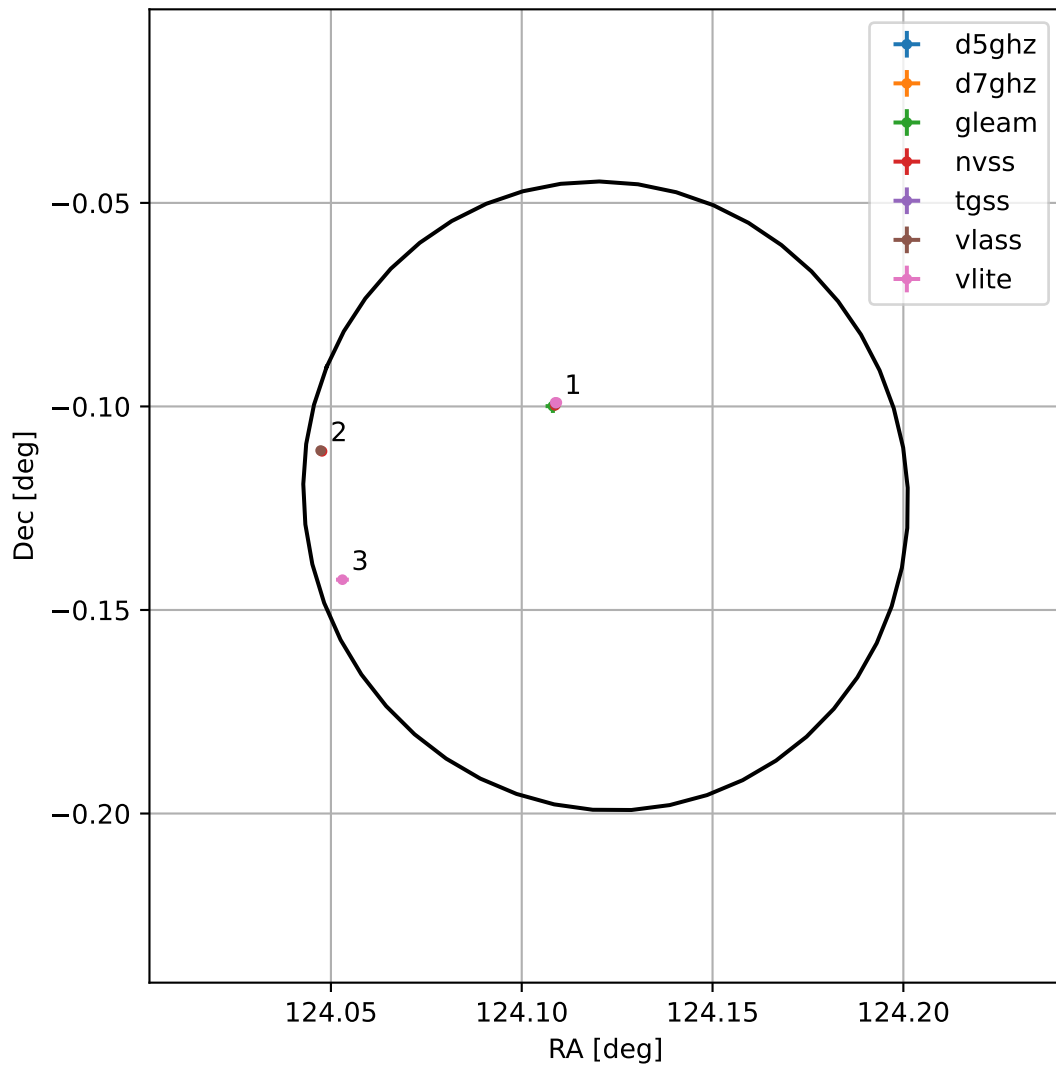
4FGL J0816.4-0007
