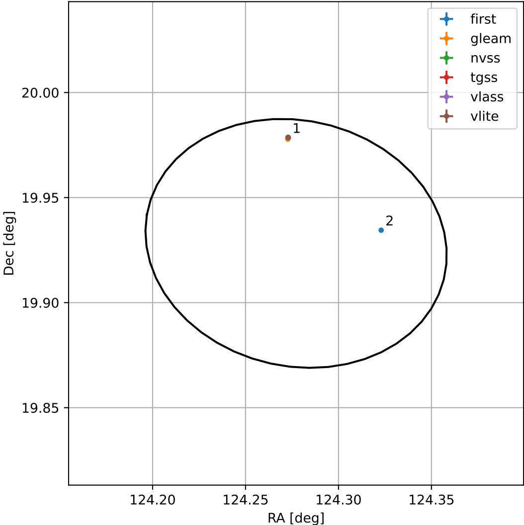
4FGL J0817.1+1955
