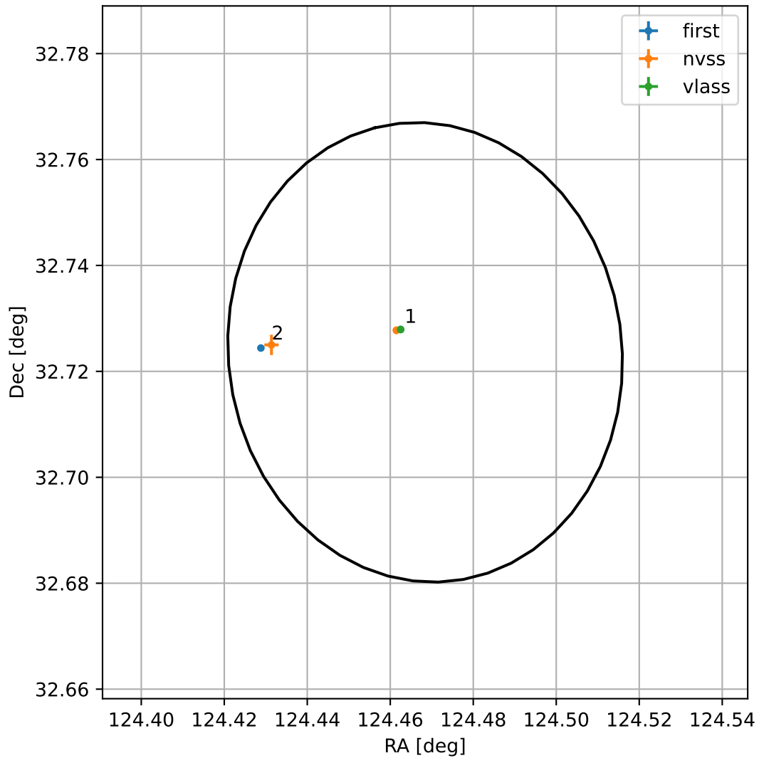
4FGL J0817.8+3243
