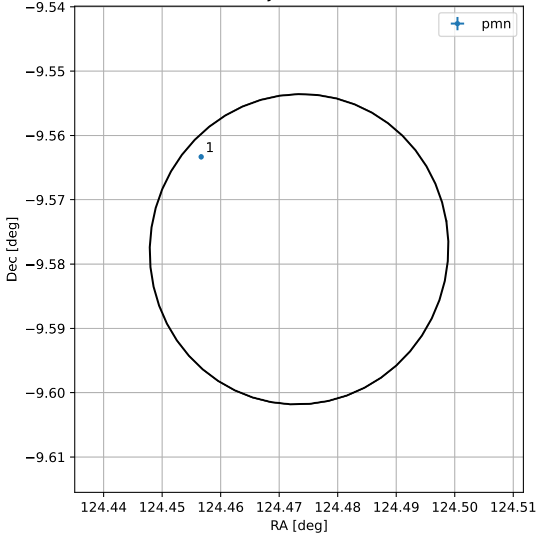
4FGL J0817.8-0934
