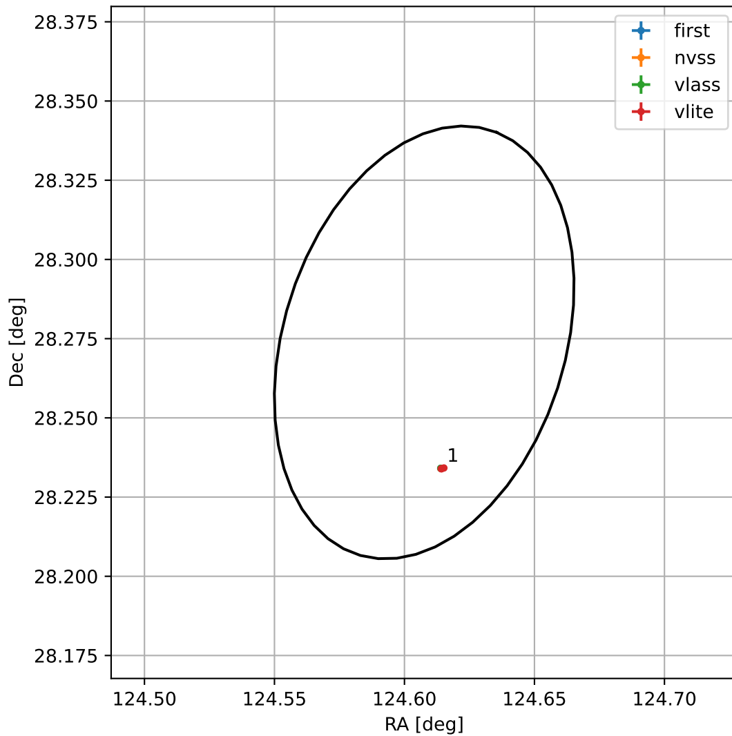
4FGL J0818.4+2816
