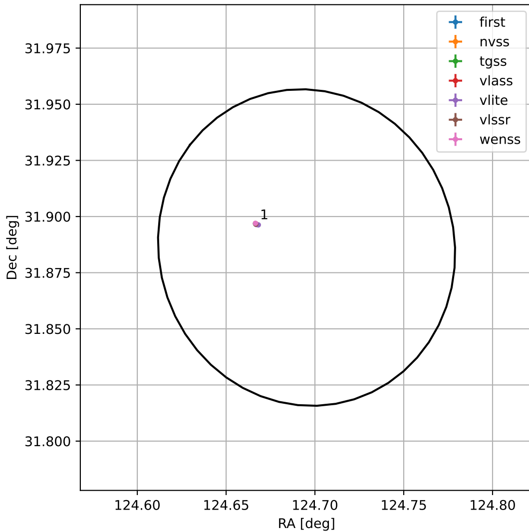
4FGL J0818.7+3153
