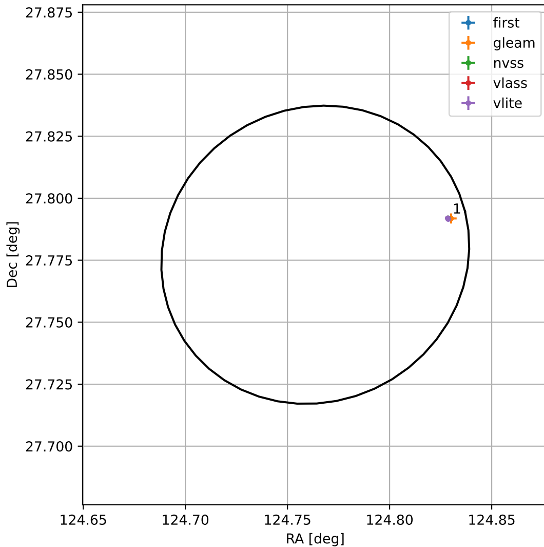
4FGL J0819.0+2746
