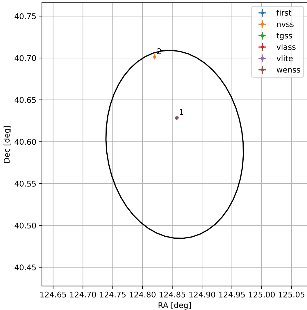
4FGL J0819.4+4035
