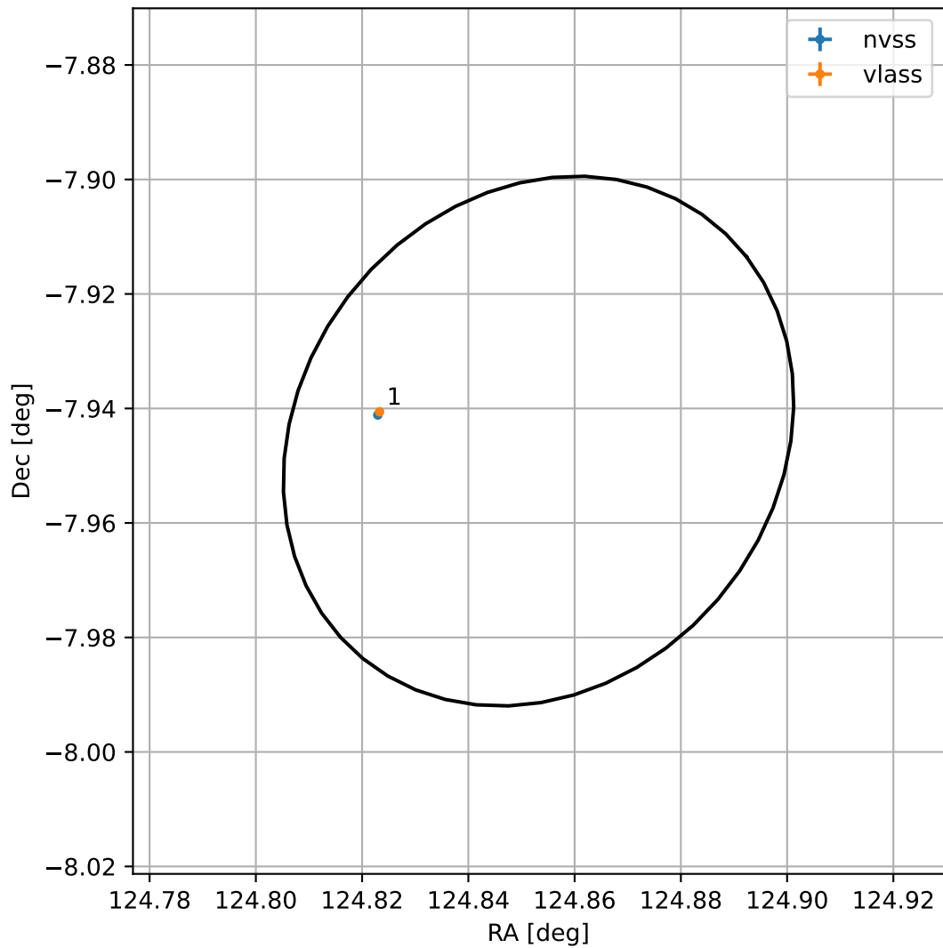
4FGL J0819.4-0756
