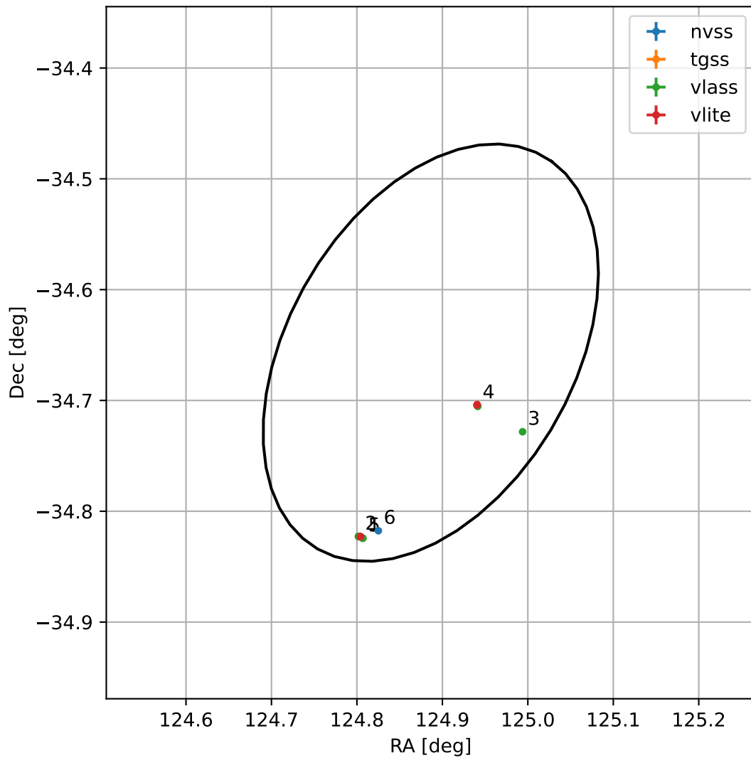
4FGL J0819.5-3439
