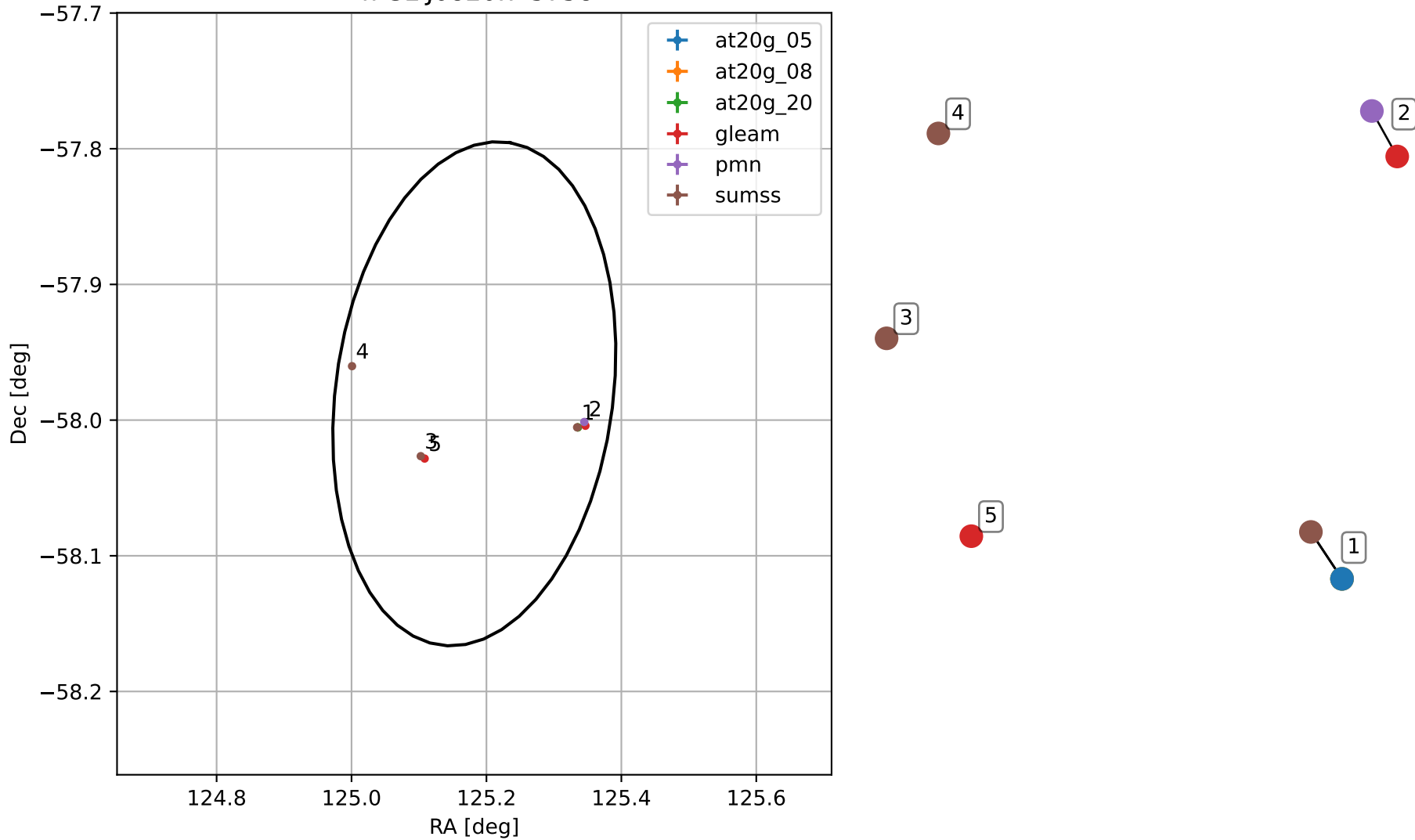
4FGL J0820.7-5758
