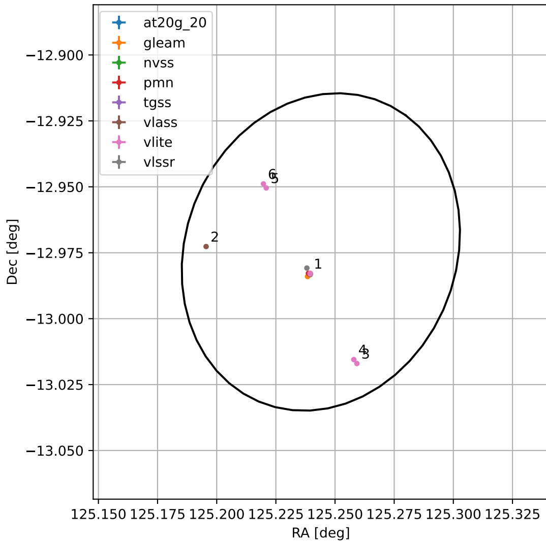
4FGL J0820.9-1258
