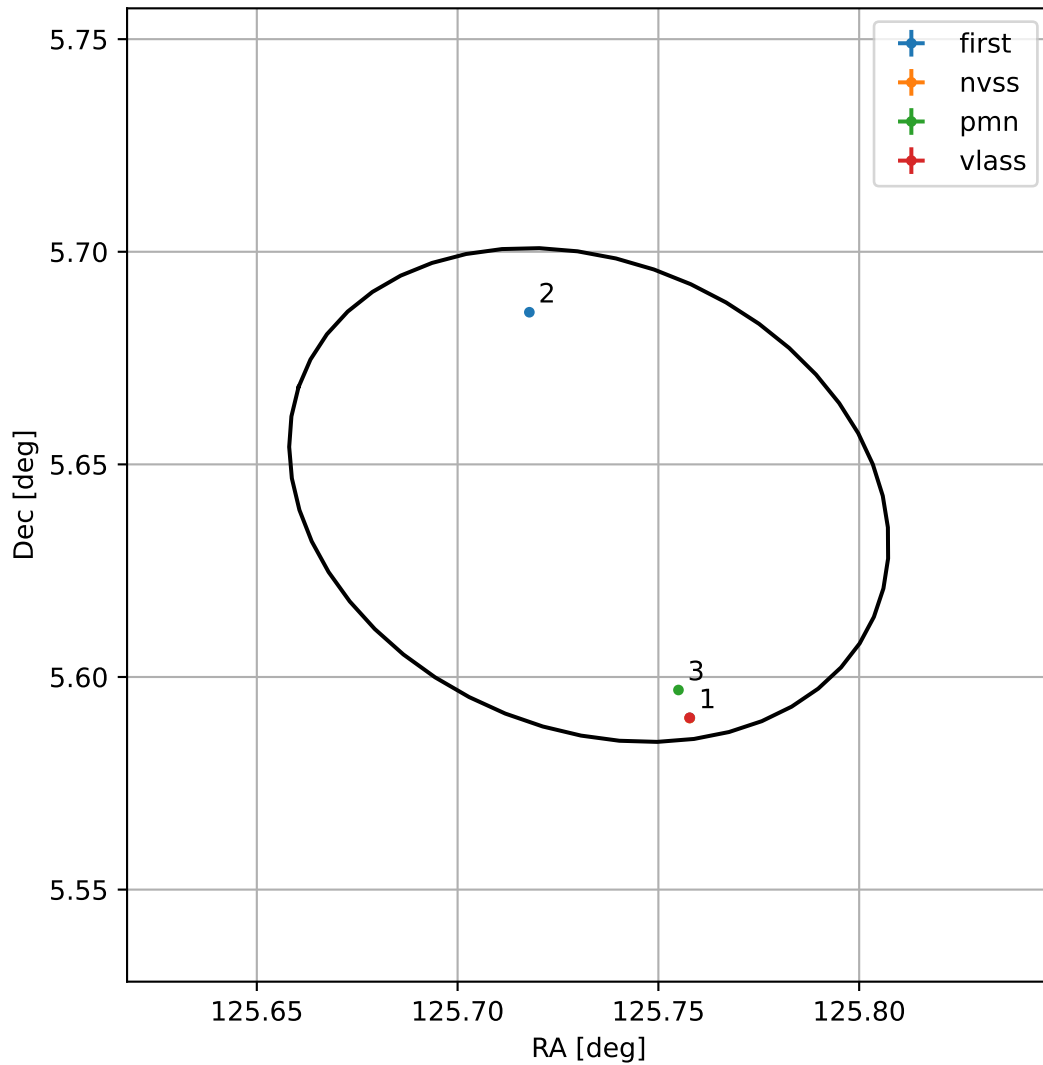
4FGL J0822.9+0538
