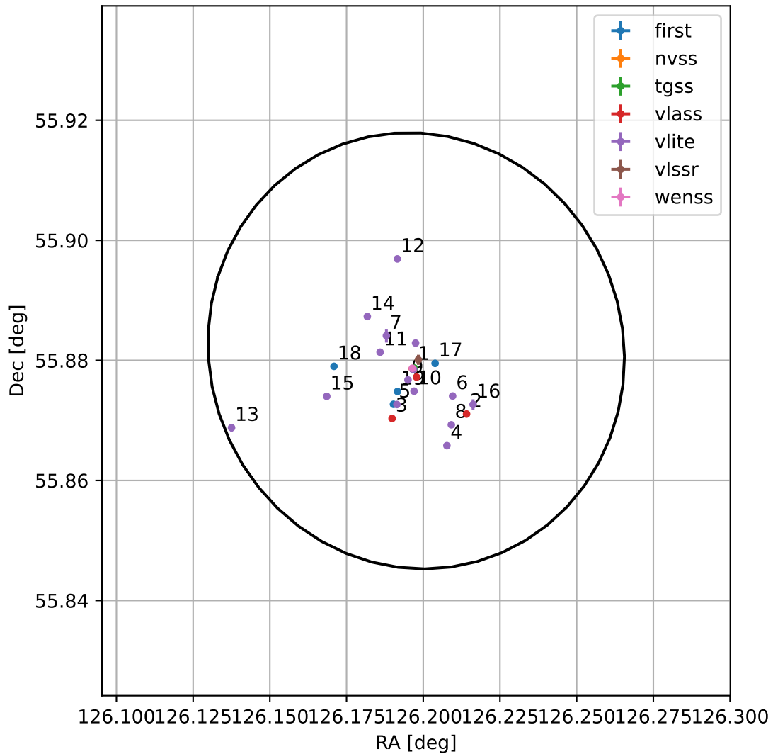
4FGL J0824.7+5552
